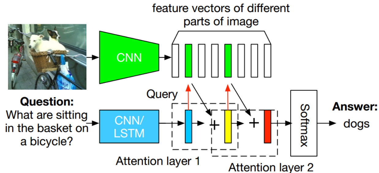
Attention Mechanism
