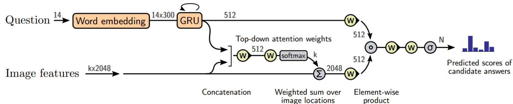
Top-Down Strategy
